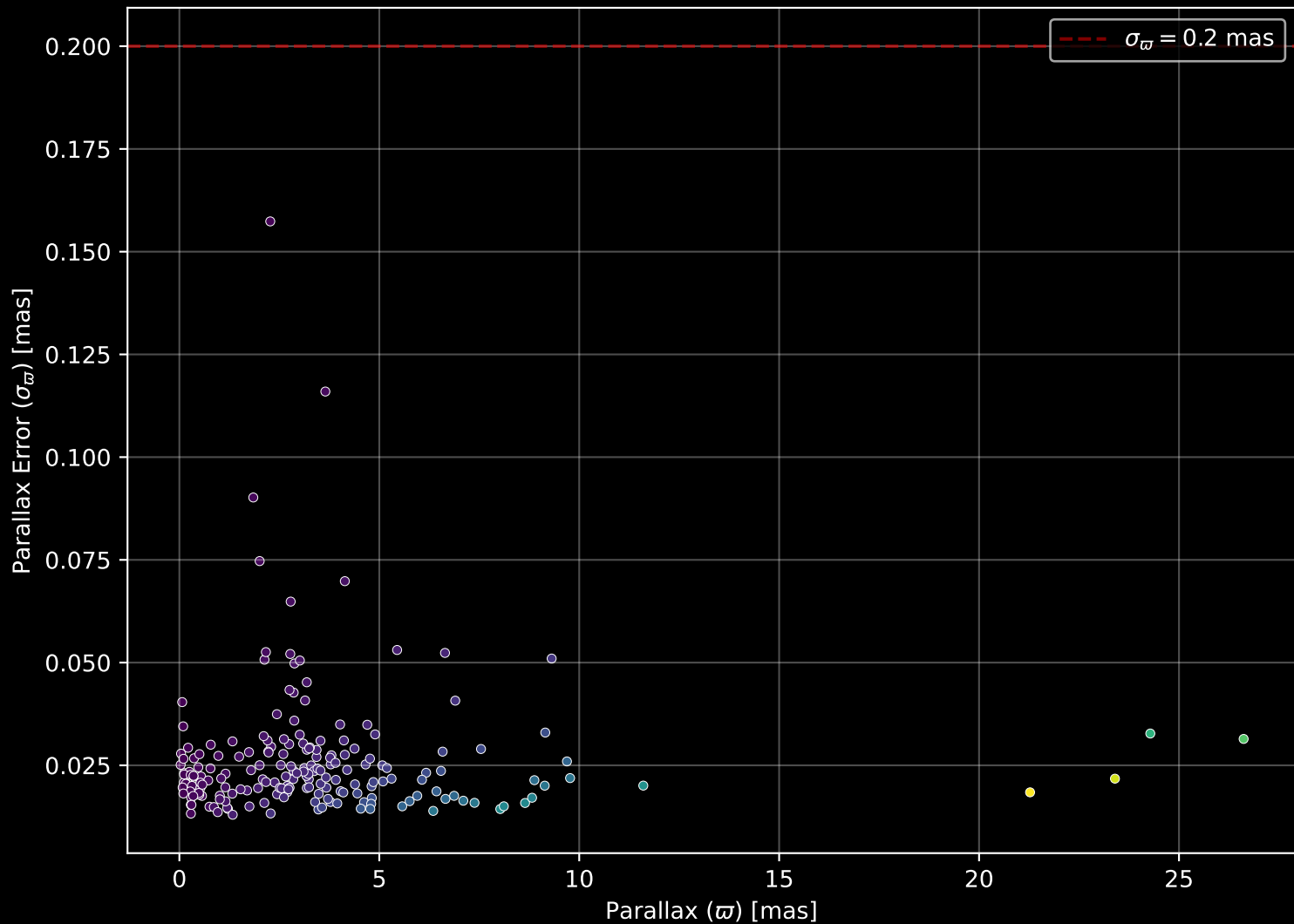
APOGEE DR17 Field: [253+75] Parallax Quality (n= 195)
