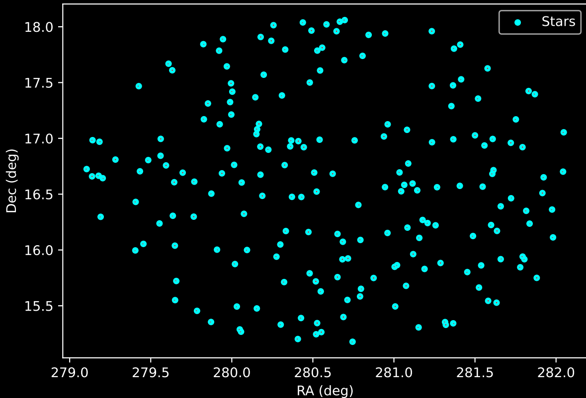
APOGEE DR17 Field: [253+75] Proper Motion Vectors for Gaia Star Field (n= 195)
