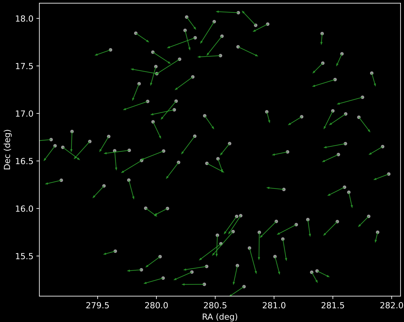
APOGEE DR17 Cluster 4 Proper Motion Vectors (n=88)
