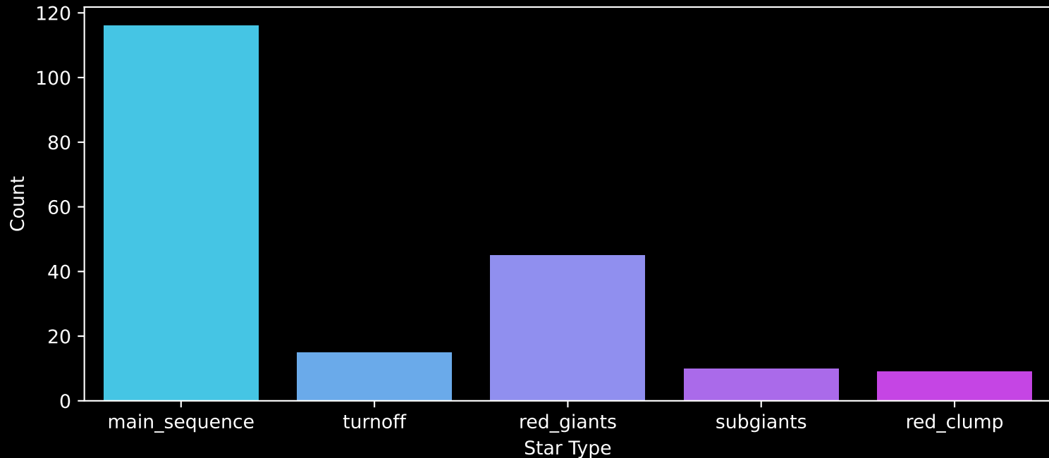
APOGEE DR17 Field: [253+75] Count plot of Star Type
