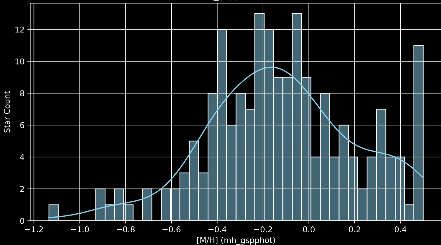
APOGEE DR17 Field: [253+75 [M/H] (mh_gspphot) (n= 189)
