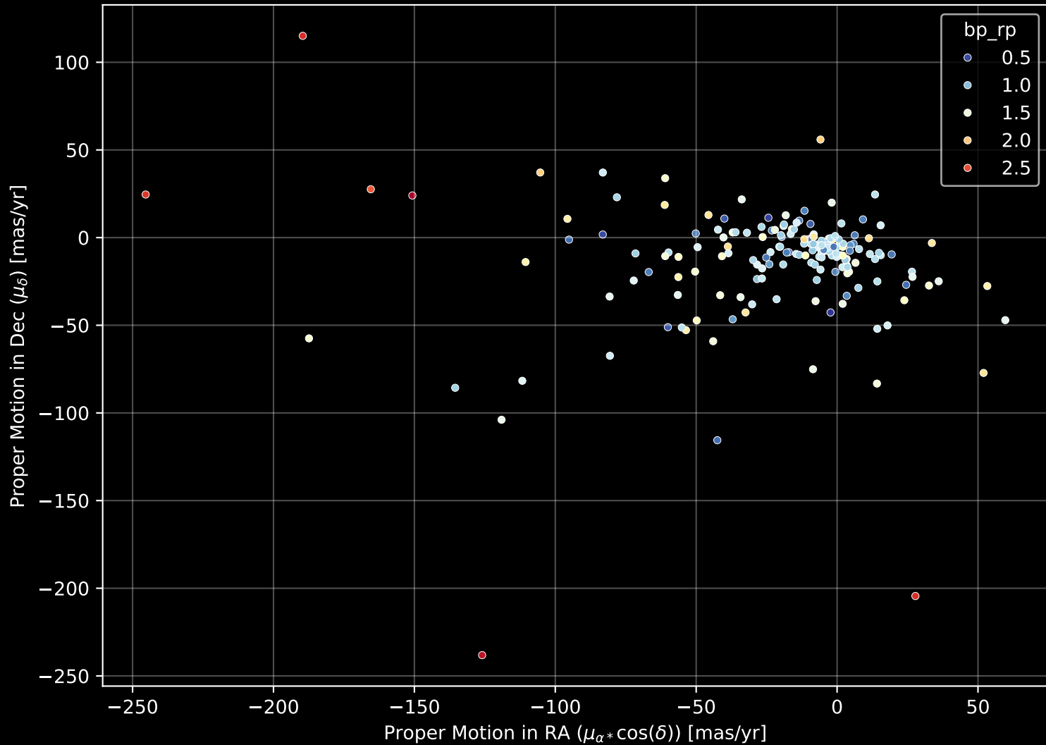
APOGEE DR17 Field: [253+75] Proper Motion Diagram (n= 195)
