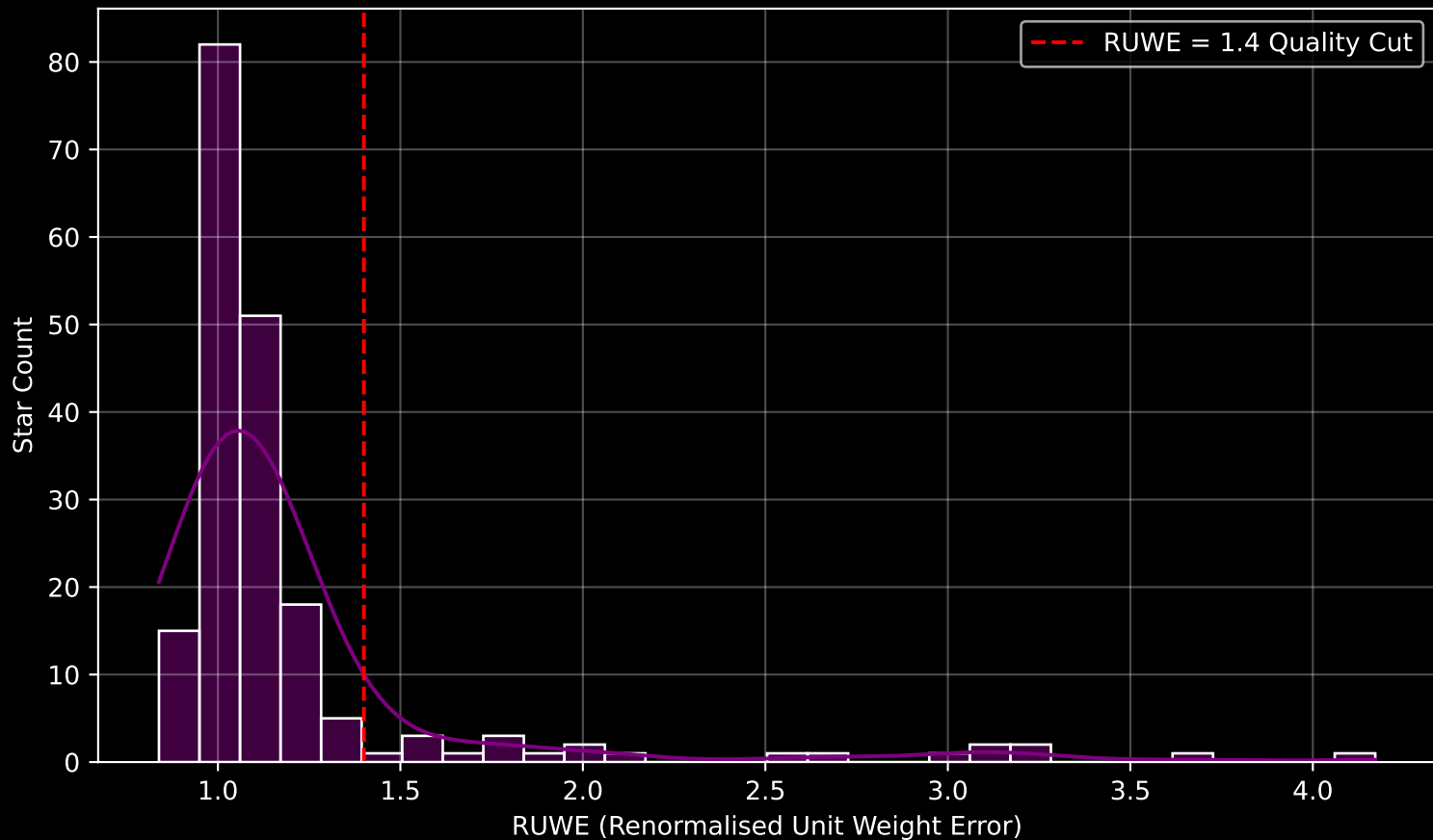
GAPOGEE DR17 Field [253+75] RUWE Distribution (n= 192)
